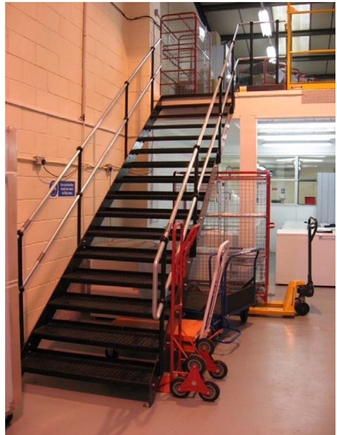
Four examples of different types of RDA Part K staircases – With open back risers, durbar steel plate treads, fully welded RHS handrails or RHS posts with galvanized steel tube handrails
